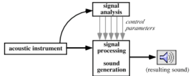
Figure 2: Electroacoustic instrument
