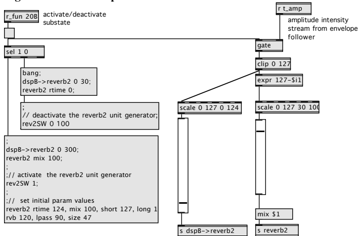
Figure 4: Code example of a "sub state"
